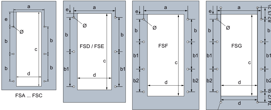
开口和钻孔尺寸 - mm (in)
